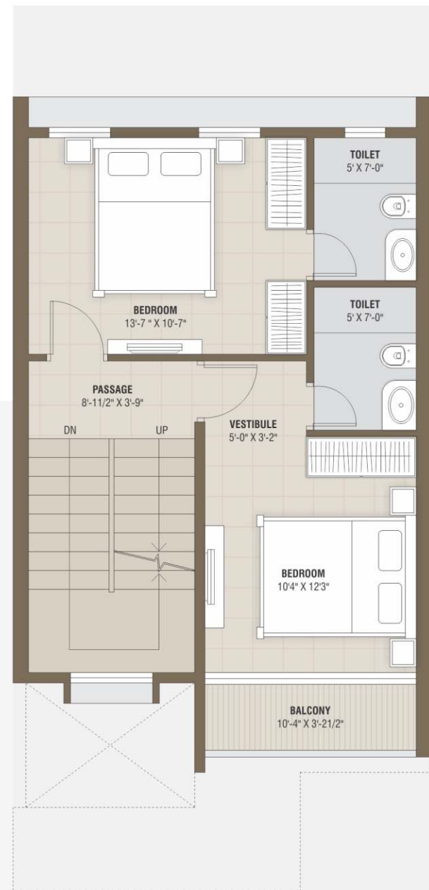
E1 & E - FIRST FLOOR PLAN
